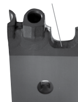
Weld chamfers around block pockets increase weld strength.
